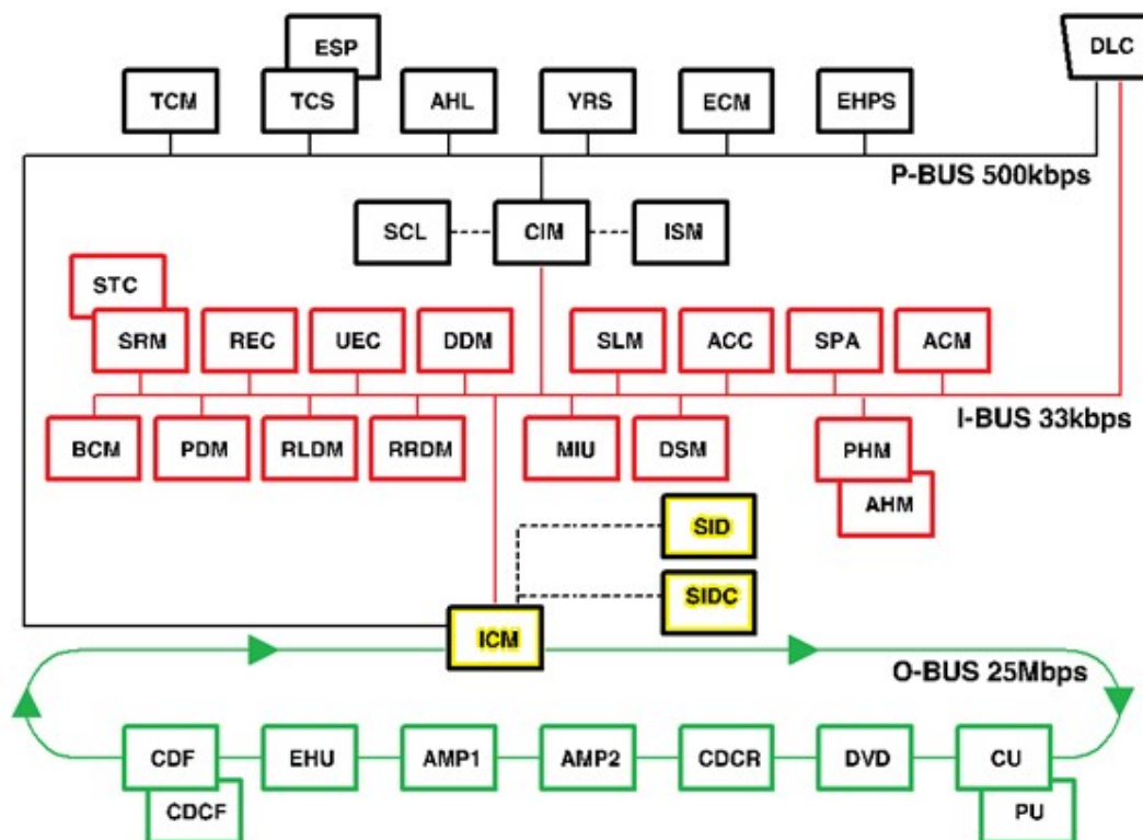
Saab 9-3 Electrical Architecture (2003-2006)
