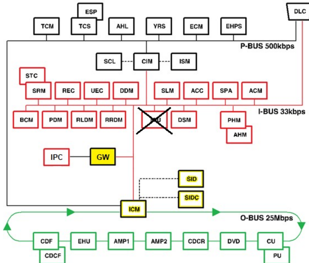
Saab 9-3 Electrical Architecture (2003-2006) with Saab NG9-5 IPC
